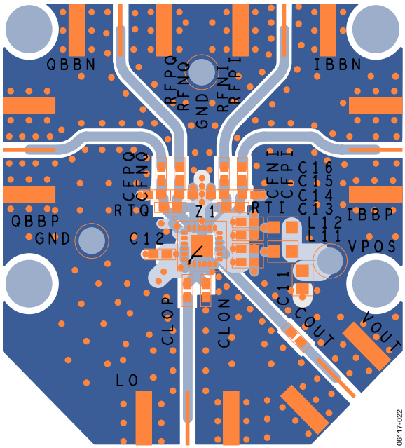
Figure 37. Evaluation Board Layout, Top Layer
